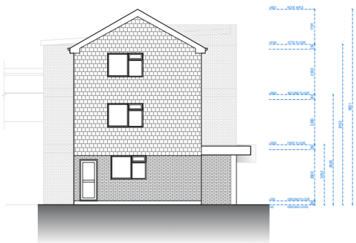
LEFT ELEVATION
